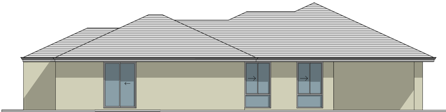
ELEVATION D
